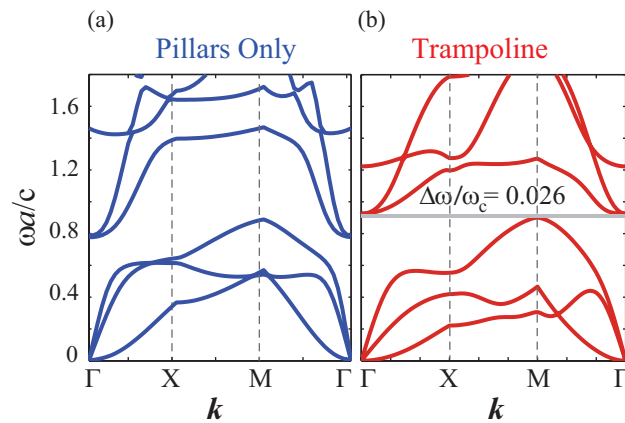
Figure 4.2: Band structure along the entire \Gamma X M \Gamma path of the irreducible Brillouin zone for cases shown in Figs. 4.1b and 4.1c. The standard pillared elastic metamaterial has no complete band gap, while the trampoline metamaterials has a band gap with a relative size of 0.026.
