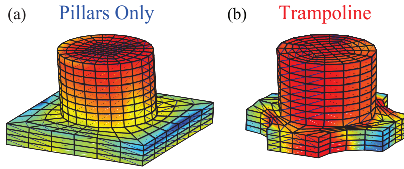
Figure 4.4: Bloch mode shapes at k_x = 0.62\pi/a for (a) standard pillared metamaterial and (b) trampoline metamaterial. The colormap represents the spatial distribution of the von Mises stress (in log scale).
