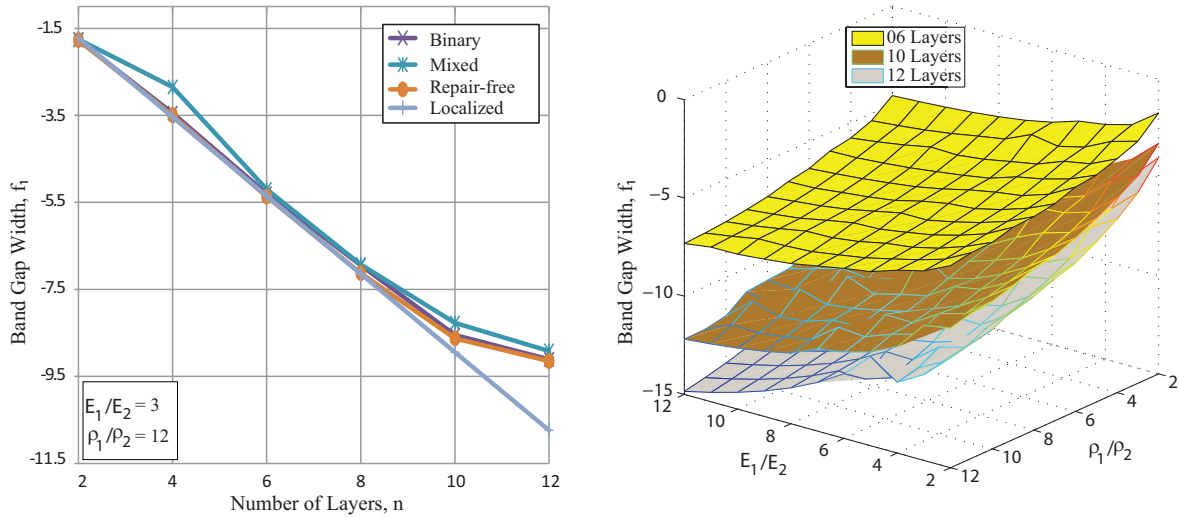
Figure 2.3: (a) Pareto diagram for the maximization of stop-band attenuation at \Omega^* = 20 for different number of layers at given ratio of \rho and E , (b) Surface plot of the same objective f_1 as a function of the ratio of material properties for 6, 10 and 12 layers.
