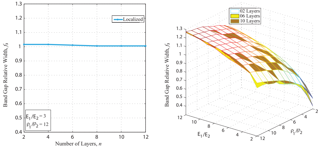
Figure 2.5: (a) Pareto diagram for the maximization of the width of the first stop-band normalized to its central frequency for different number of layers at given ratio of \rho and E , (b) Surface plot of the same objective f_3 as a function of the ratio of material properties for 2, 6 and 10 layers.
