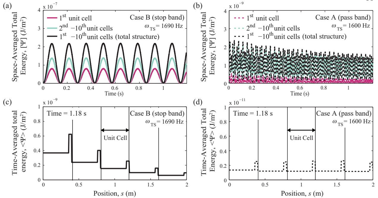
Figure 5.3: Average quantities of the total energy in the phononic subsurface for Case B ( \omega_{TS} = 1690 Hz in a stop band) and Case A ( \omega_{TS} = 1600 Hz in a pass band). The space-averaged total energy, defined as \{\Psi(\omega^*, t)\} = \int_{s=0}^{s=l} [\Psi(\omega^*, t)] ds \approx \sum_{j=1}^{j=n_s} \Psi_j^{(i)} , is shown in (a) for Case B and in (b) for Case A. The time-averaged total energy, defined as \langle \Psi(\omega^*, t) \rangle = \int_{t=0}^{t=t_T} [\Psi(\omega^*, t)] dt \approx \sum_{i=1}^{i=n} \Psi_j^{(i)} , is shown in (c) for Case B and in (d) for Case A. The unit cells are marked by vertical lines.
