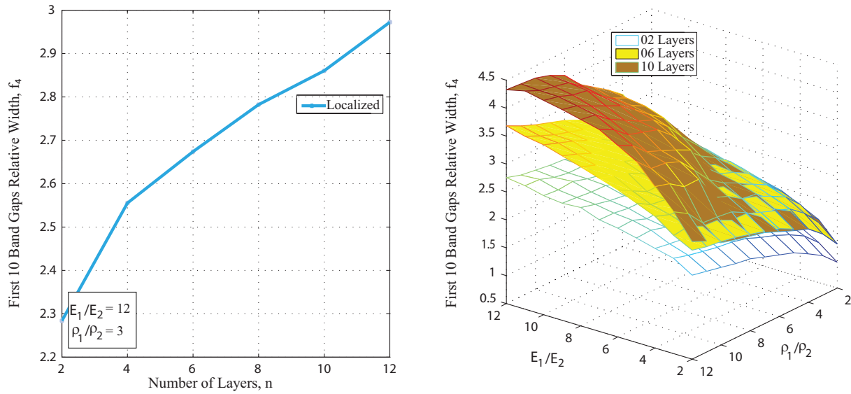
Figure 2.6: Pareto diagram for the maximization of the summation of the width of the first 10 stop-bands normalized to their central frequency for different number of layers at given ratio of \rho and E , (b) Surface plot of the same objective f_4 as a function of the ratio of material properties for 2, 6 and 10 layers.
